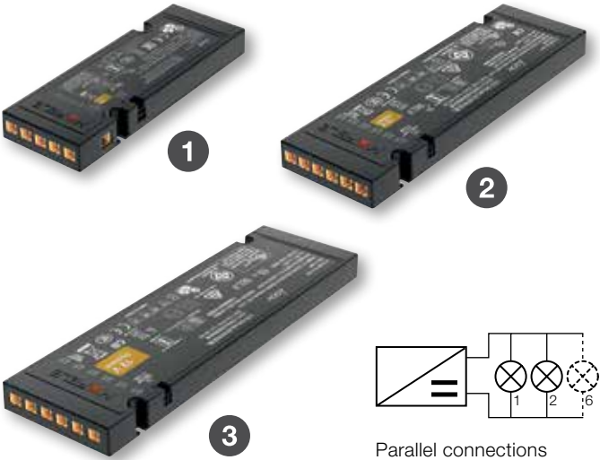
Parallel connections
