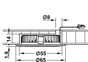
Recess mounting
